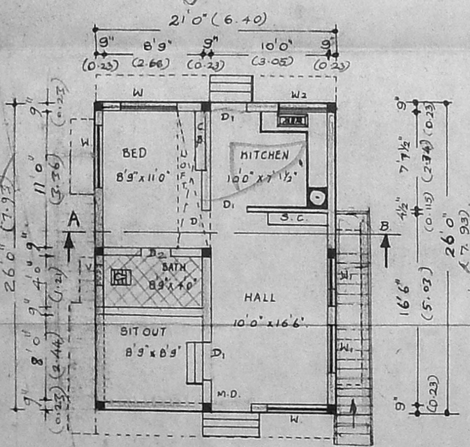
PLAN
